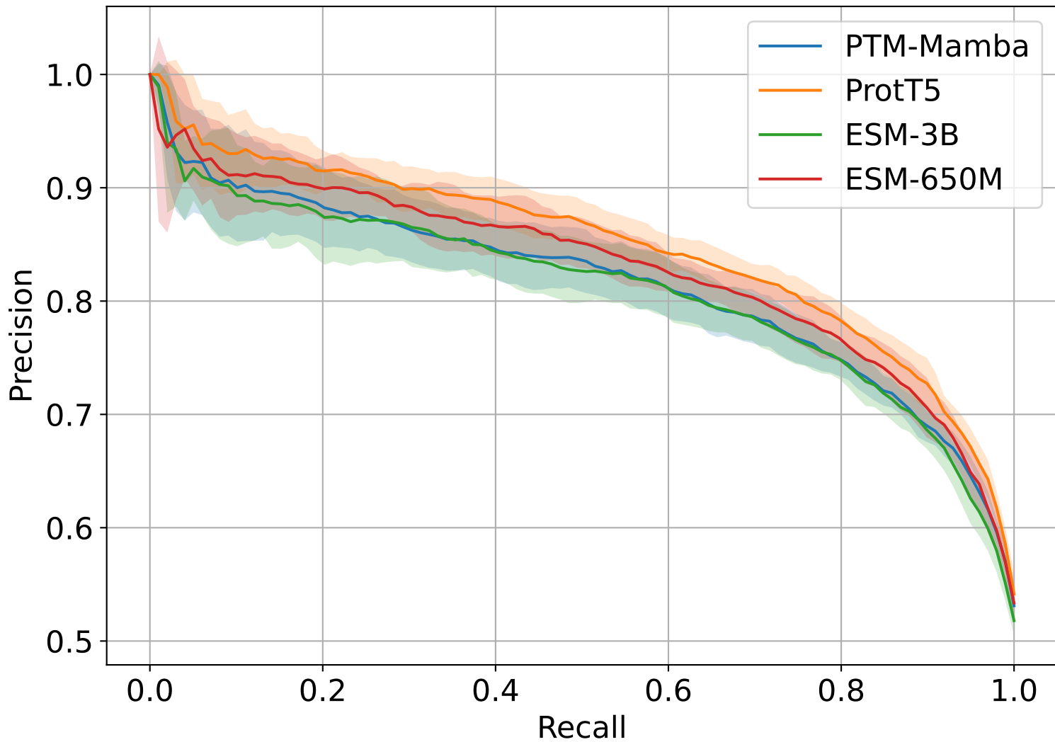
Precision-Recall Curve
